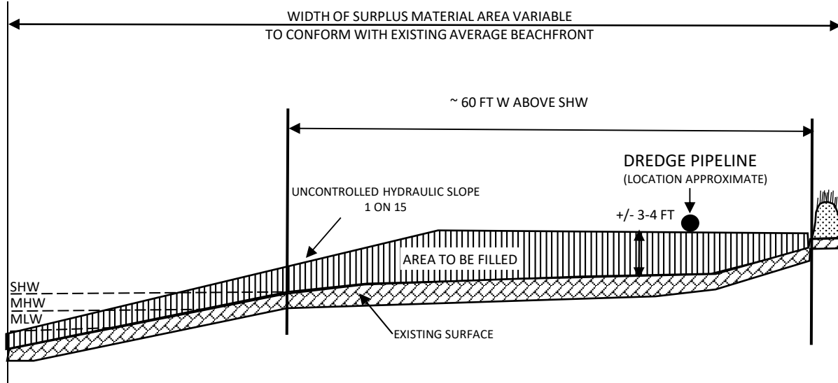
TYPICAL BEACH NOURISHMENT SECTION WADES BEACH
