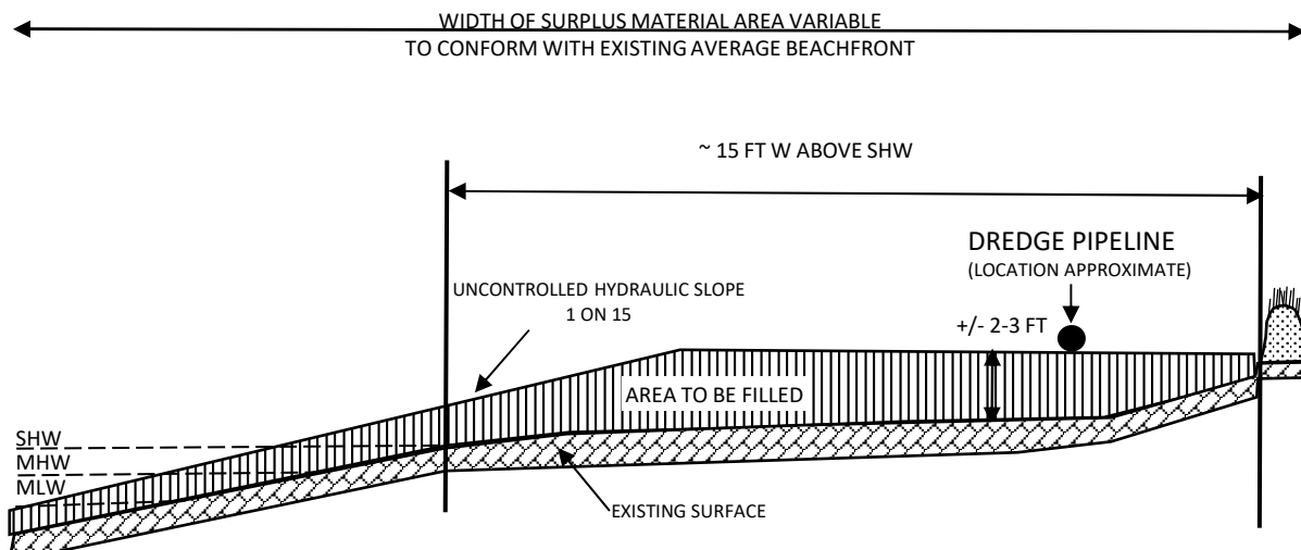
TYPICAL BEACH NOURISHMENT SECTION SHELL BEACH
