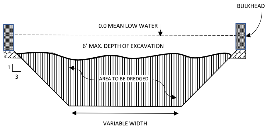
TYPICAL CHANNEL SECTION WITH BULKHEAD (UPPER CHANNEL)
